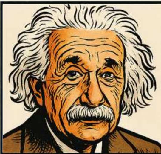
TEORIE RELATIVITY
